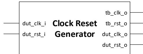
Figure 2.1. Clock Reset Generator Block Diagram
