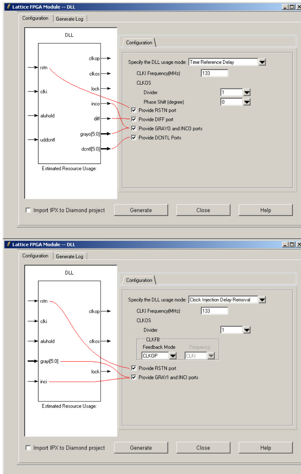
Figure 10-42. Diamond LatticeECP3 IPexpress DLL Configuration Tab (see Figure 10-22 for ispLEVER Equivalent)
