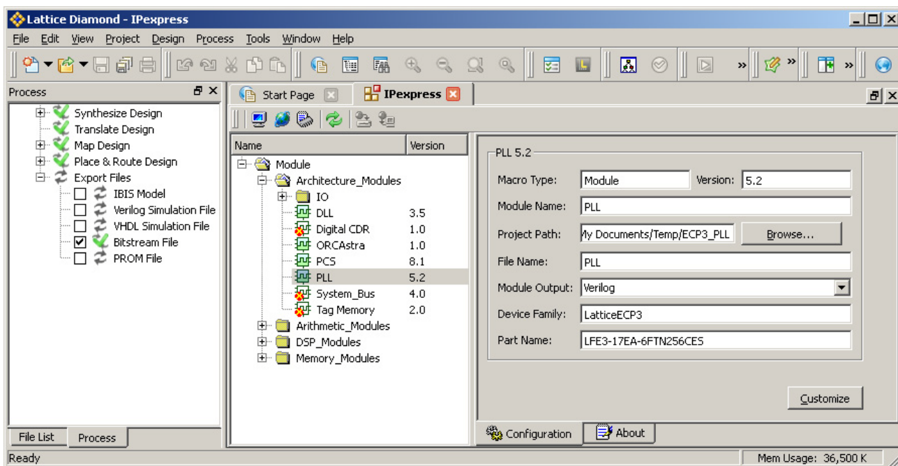
Figure 10-40. Diamond IPexpress Main Window (see Figure 10-14 for ispLEVER Equivalent)
