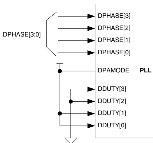
Figure 10-11. Example of Dynamic Phase Adjustment with a Fixed Duty Cycle of 3/16th of a Period
