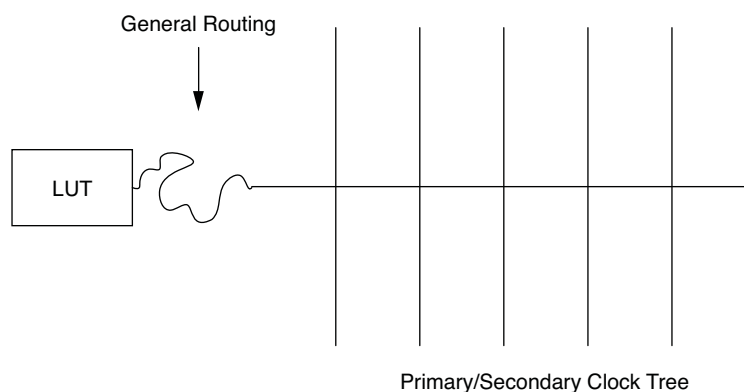
Figure 10-3. General Routing Connection to Dedicated Clock Resource from LUT
