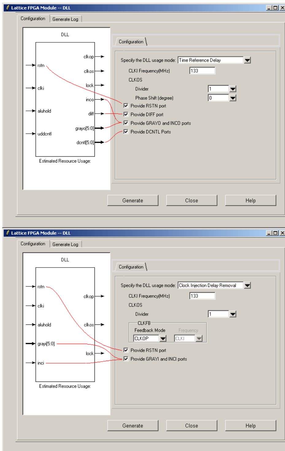
Figure 10-22. ispLEVER LatticeECP3 IPexpress DLL Configuration Tab (see Figure 10-42 for Diamond Equivalent)
