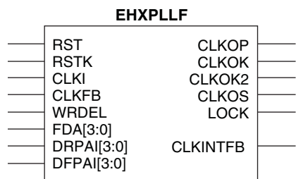
Figure 10-13. LatticeECP3 PLL Library Symbol
