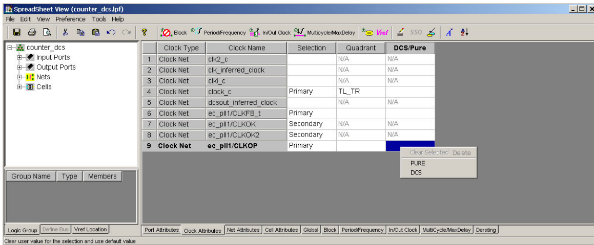
Figure 10-6. ispLEVER Design Planner Spreadsheet View (see Appendix C Figure 10-39 for Diamond Equivalent)
