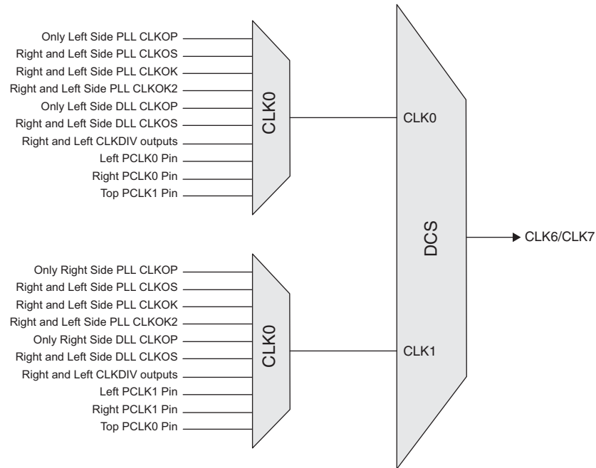
Figure 10-36. Dedicated DCS Clock Sources
