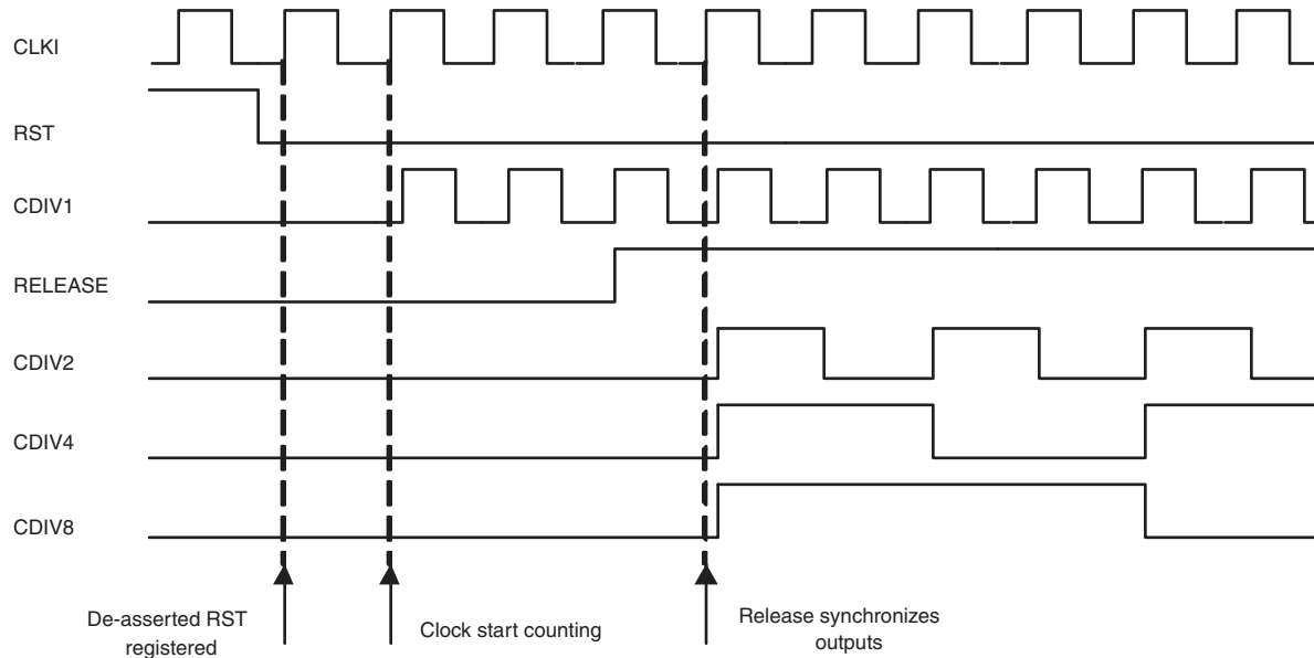
Figure 10-28. CLKDIV Release Behavior
