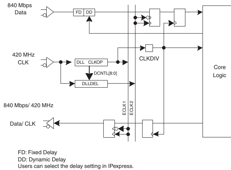
Figure 10-24. SPI4.2 and DDR Registers Interface Application
