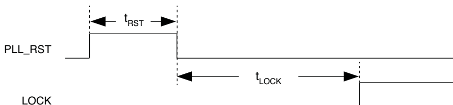
Figure 10-8. RST Input Timing Diagram
