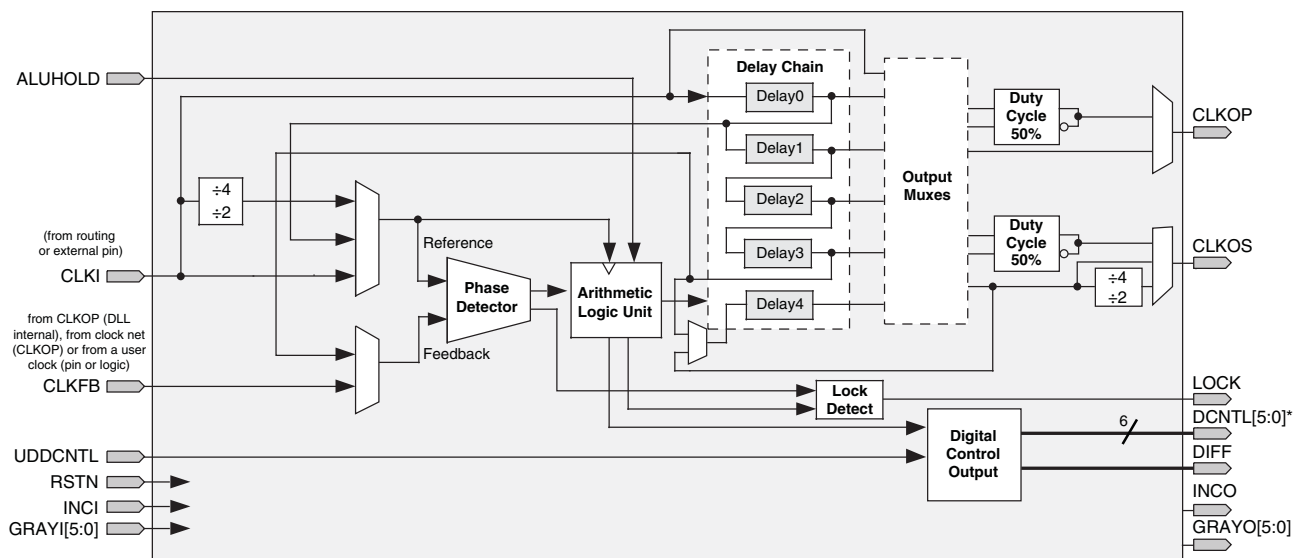
Figure 10-18. LatticeECP3 DLL Block Diagram
