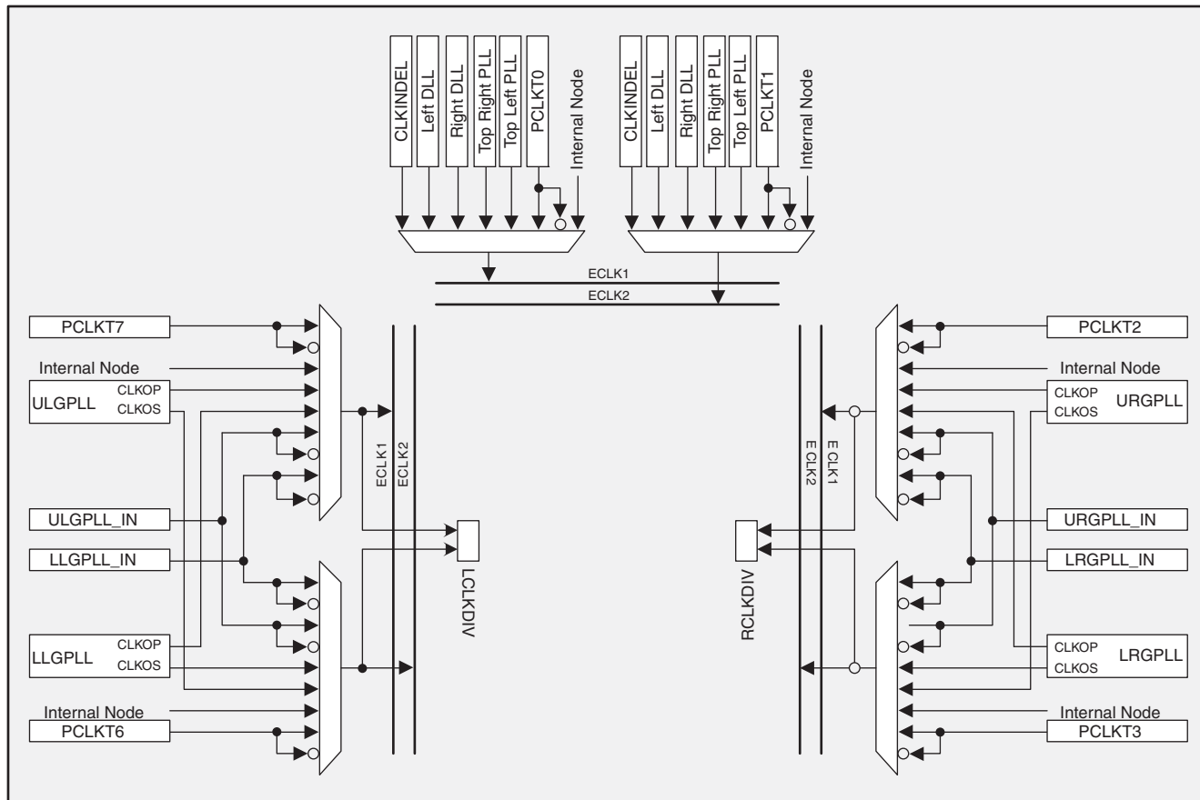
Figure 10-37. PLL, CLKIDV and ECLK Locations and Connectivity
